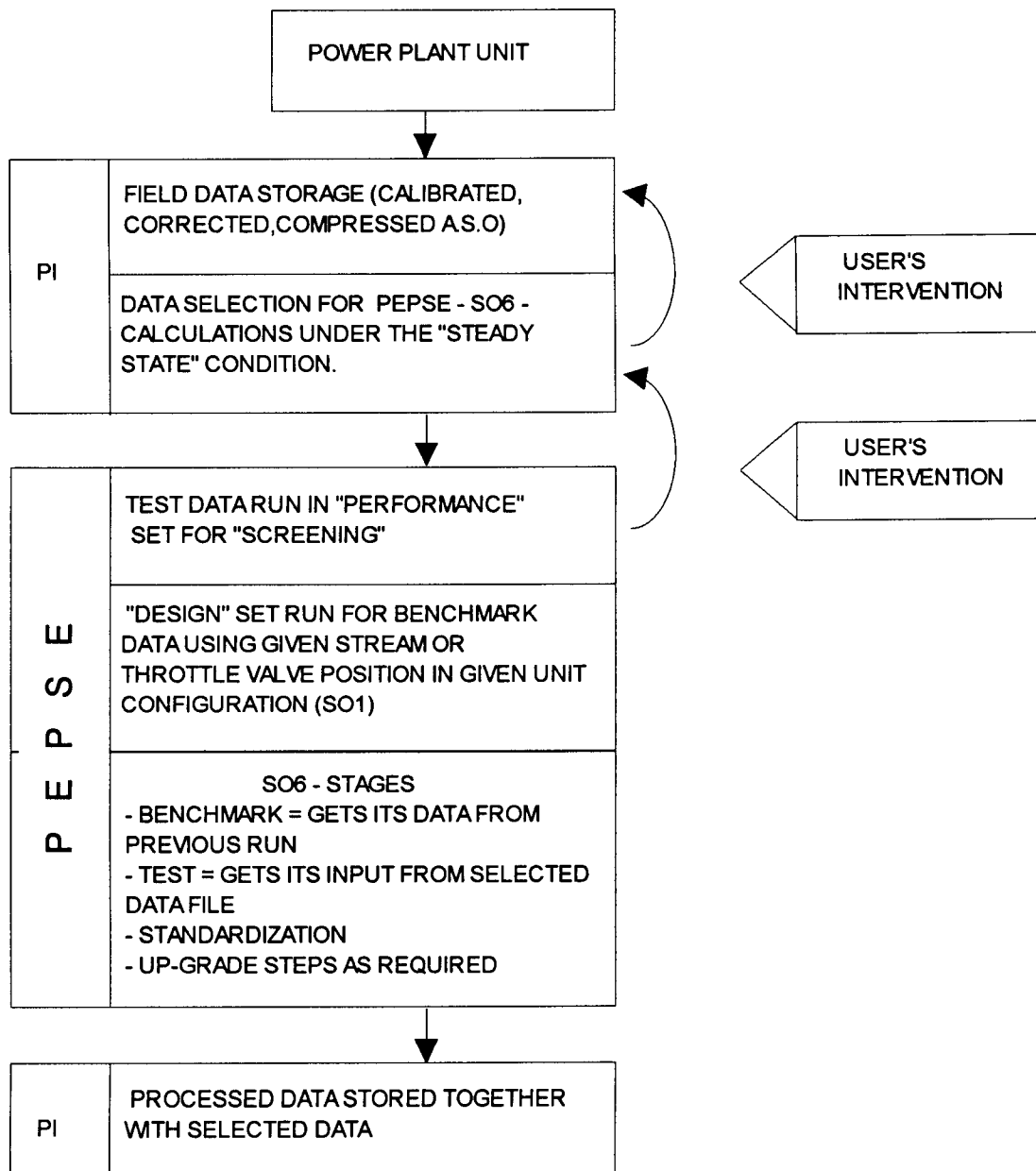
FIG.1 Flow chart for I.E.C.'S procedure for the processing of stored field data using PEPSE.
